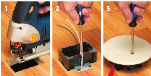
Adjustable boxes for varying floor heights
